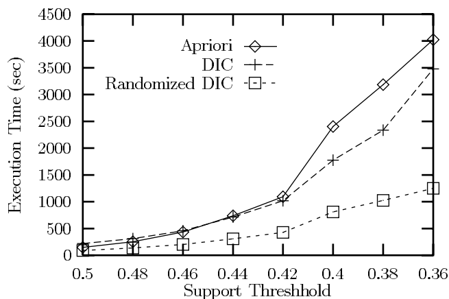
Figure 9: Performance of Apriori and DIC on Census Data
