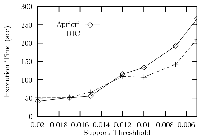
Figure 8: Performance of Apriori and DIC on Synthetic Data
