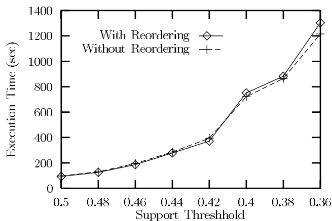
Figure 11: Performance With and Without Item Reordering
